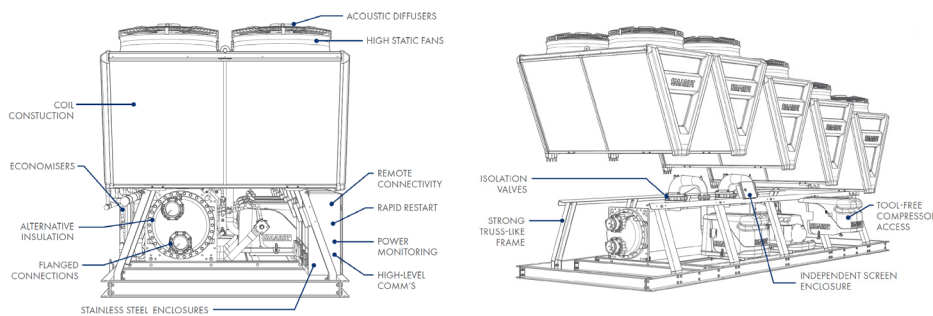
Side and front views of a Smardt T-Class AD Design Series chiller
